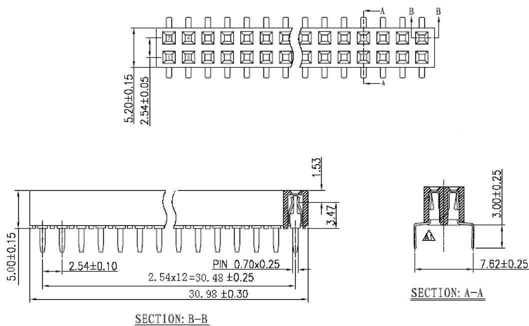
Figure 2 Drawing of Electrical Connector
