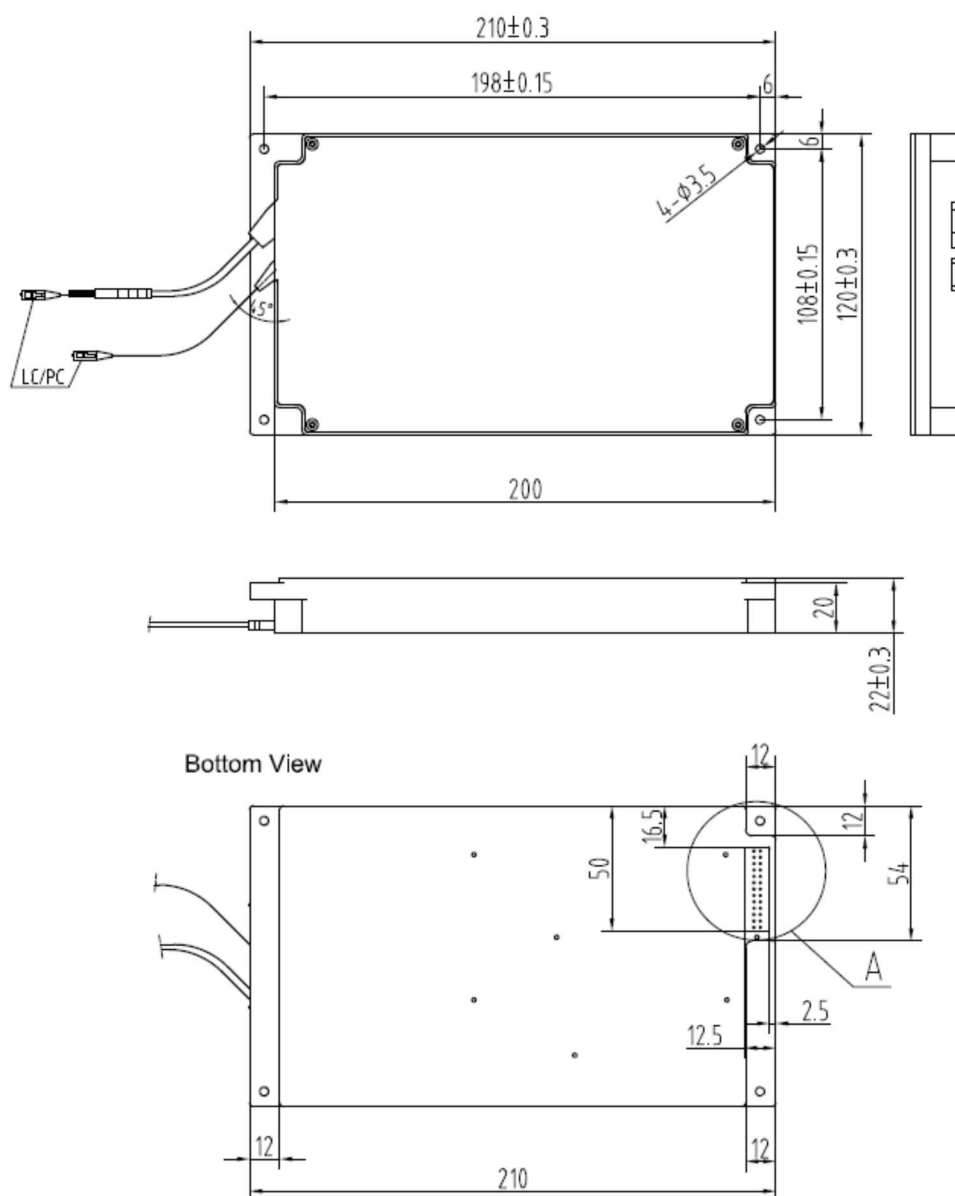
Figure 3 Mechanical Drawings of VMUX
