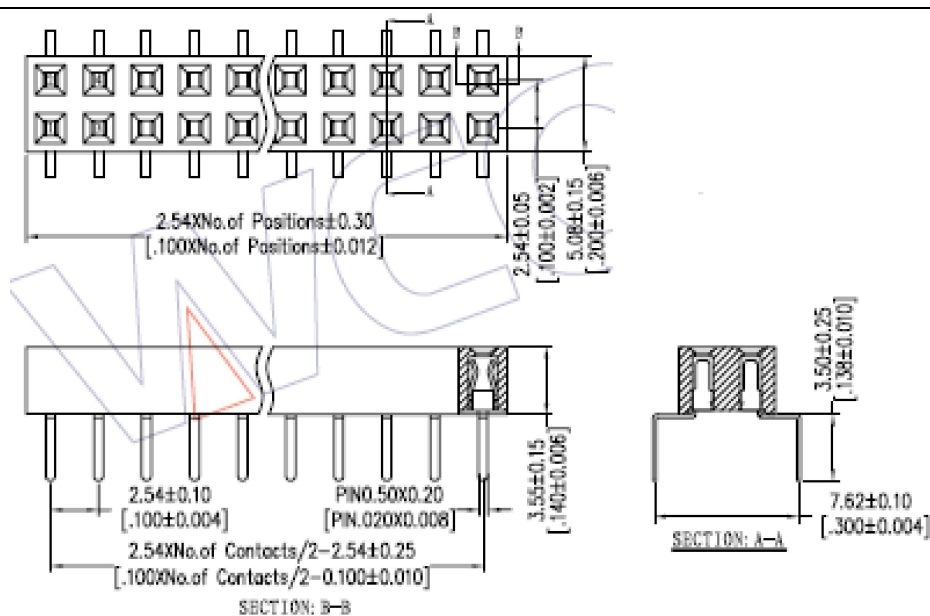
Figure 2 Drawing of Electrical Connector
