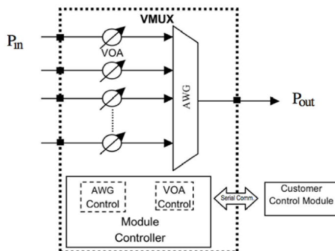
Figure 1 Functional Scheme (VMUX)
