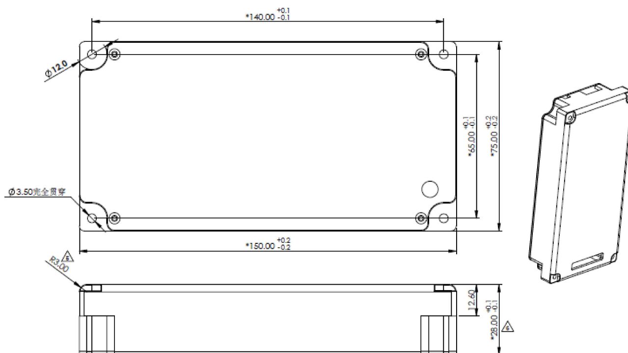
Figure 3 Mechanical Drawings of VMUX
