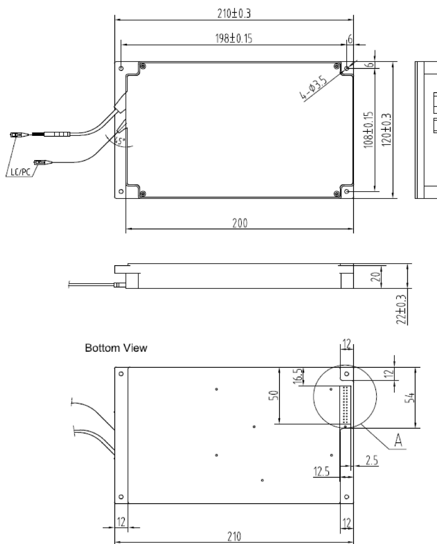
Figure 3 Mechanical Drawings of VMUX
