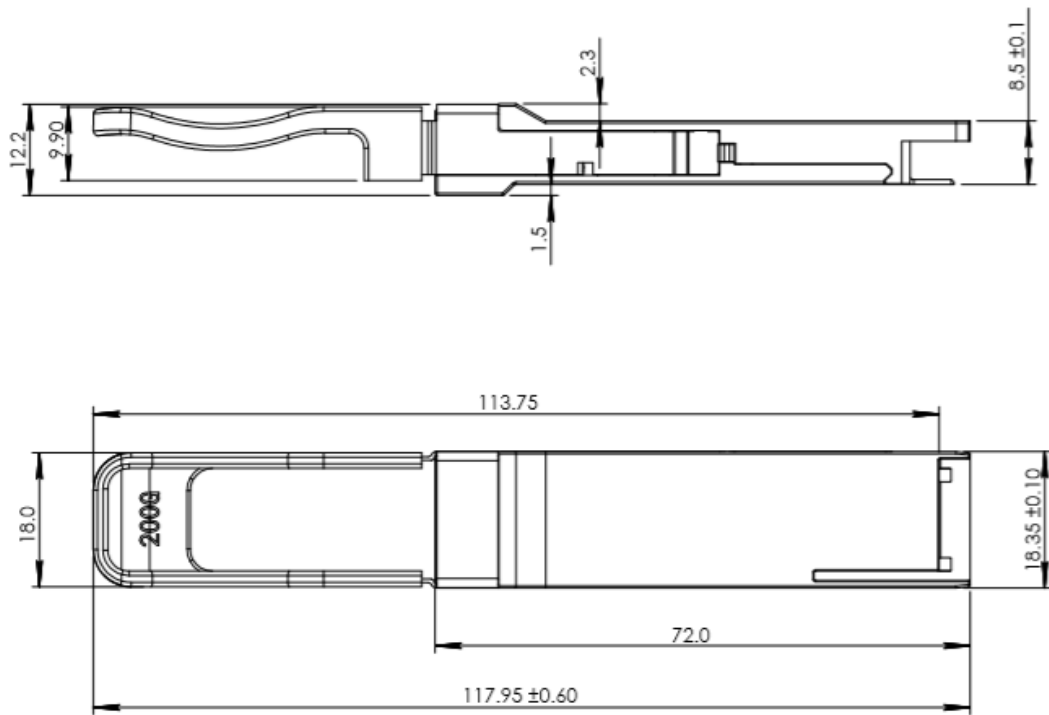
Figure 4. Mechanical Outline
