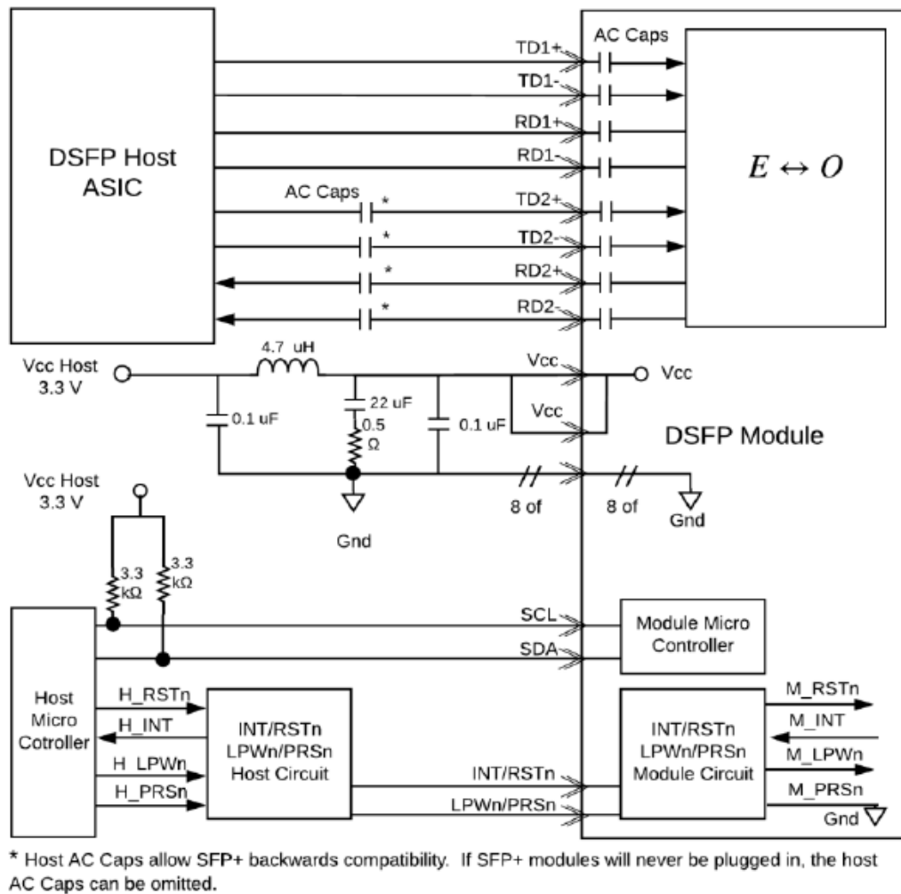
Figure 1: Recommended Host Board Power Supply Filtering
