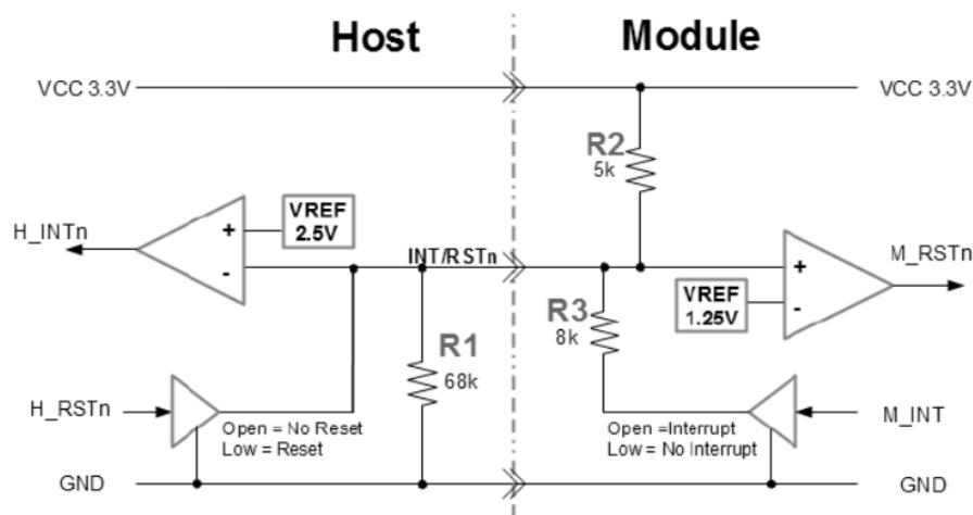
Figure 2: INT/RSTn circuit
